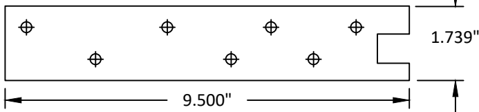
30 INACTIVE LOCK SIDE REINF. PLATE ALUMINUM
