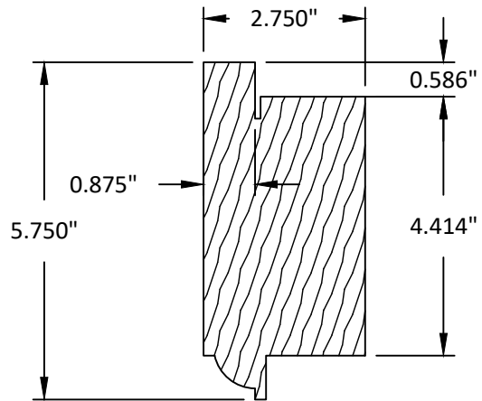
6 OFFSET HINGE STILE AND TOP RAIL WOOD
