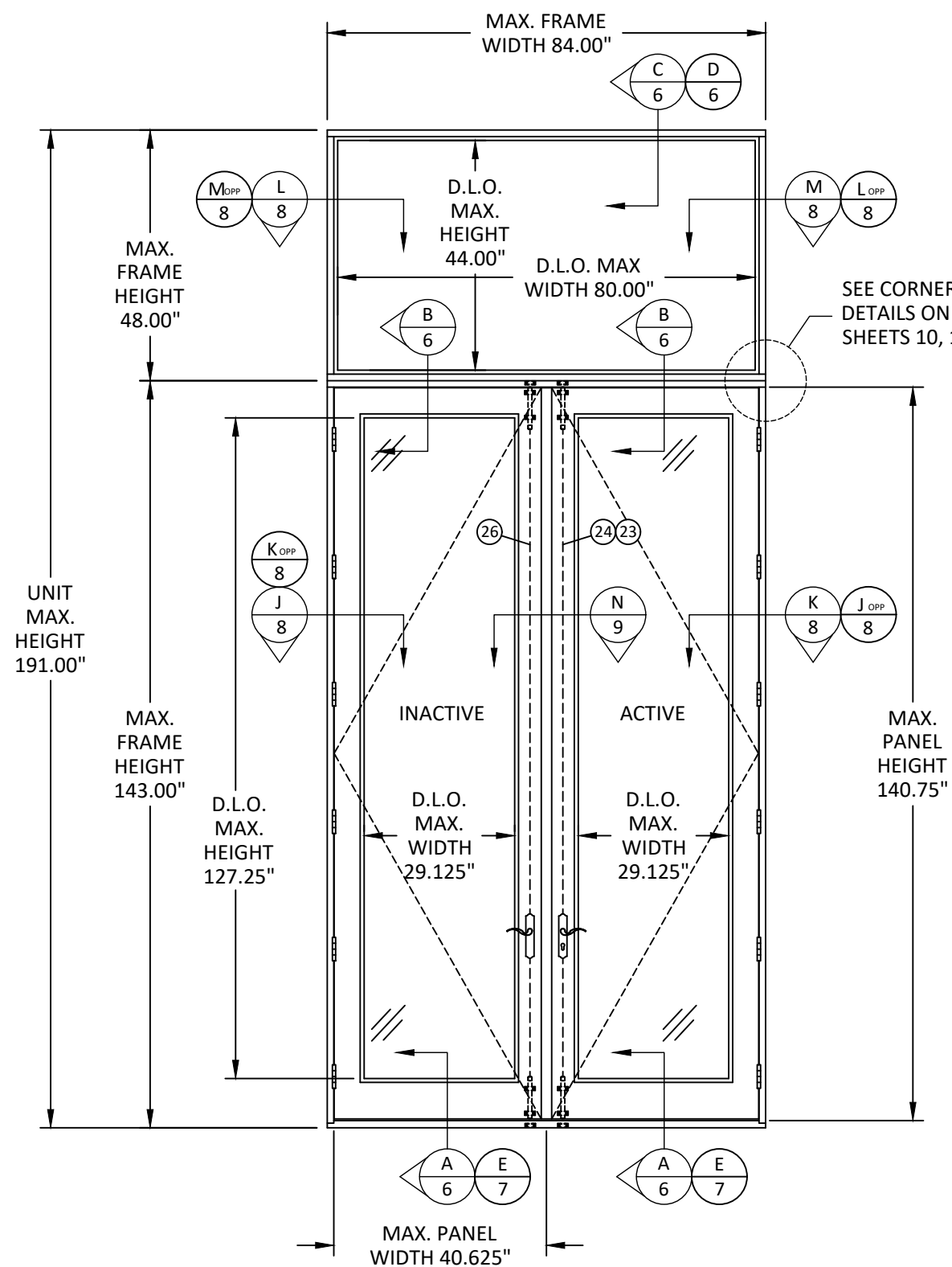
EXTERIOR ELEVATION (OUTSWING DOORS)
