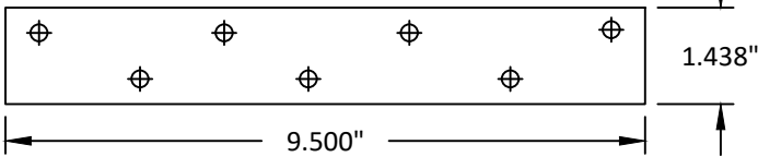
28 HINGE SIDE REINF. PLATE ALUMINUM
