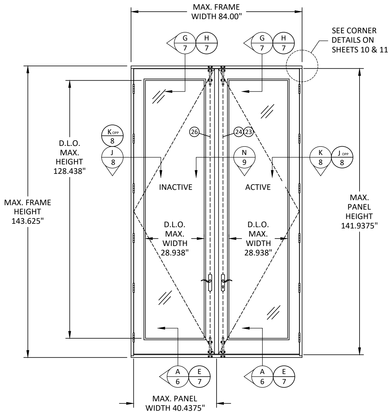
EXTERIOR ELEVATION (OUTSWING DOORS)
