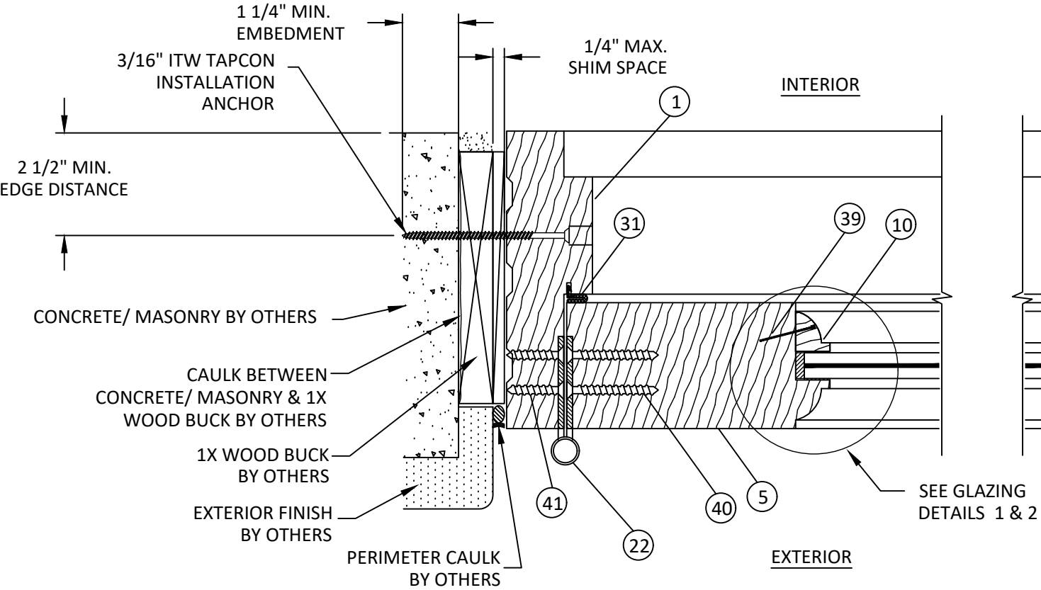
J 8 HORIZONTAL SECTION JAMB AT CONCRETE/MASONRY
