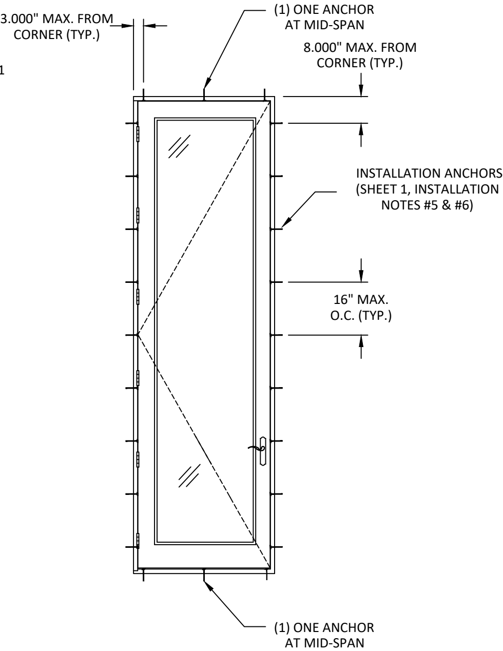
ANCHOR LAYOUT
