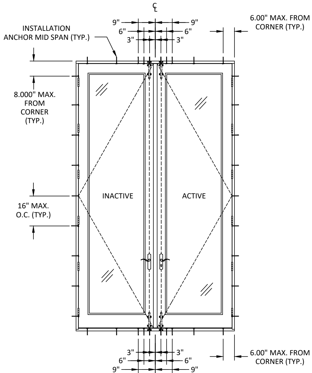
ANCHOR LAYOUT
