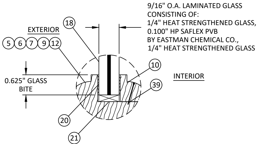
GLAZING DETAIL 1
