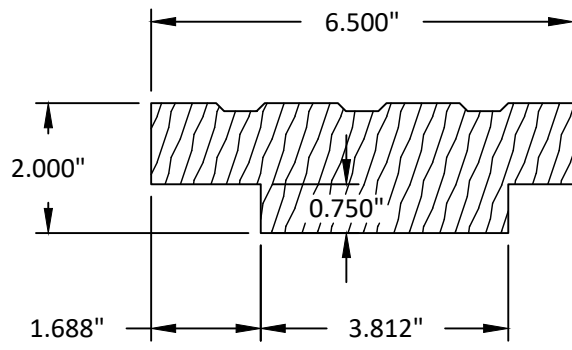
7 BOTTOM RAIL WOOD
