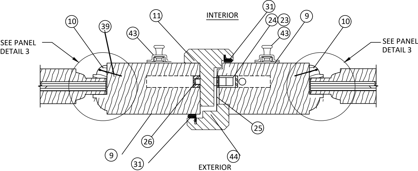
M 9 RAISED PANELS HORIZONTAL SECTION MEETING STILES
