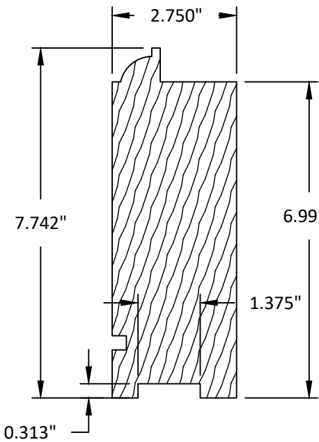
13 WEATHER STRIP GUIDE WOOD
