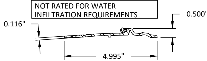
15 ADA THRESHOLD EXTRUDED ALUMINUM
