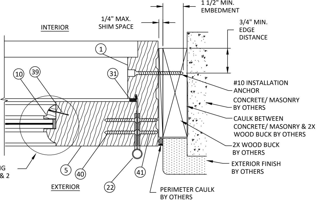
K 8 HORIZONTAL SECTION JAMB AT 2X WOOD BUCK
