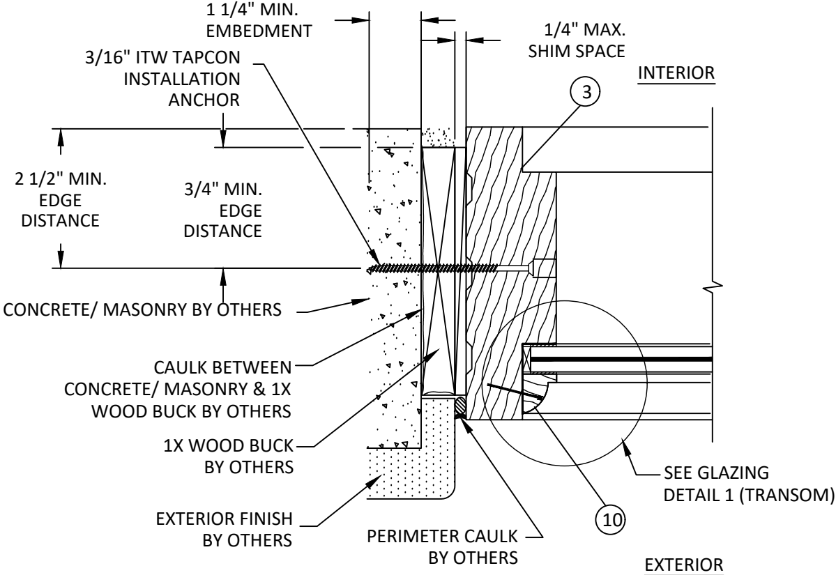
L 8 HORIZONTAL SECTION JAMB/TRANSOM AT CONCRETE/MASONRY
