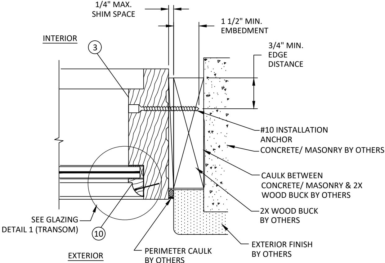
M 8 HORIZONTAL SECTION JAMB/TRANSOM AT 2X WOOD BUCK
