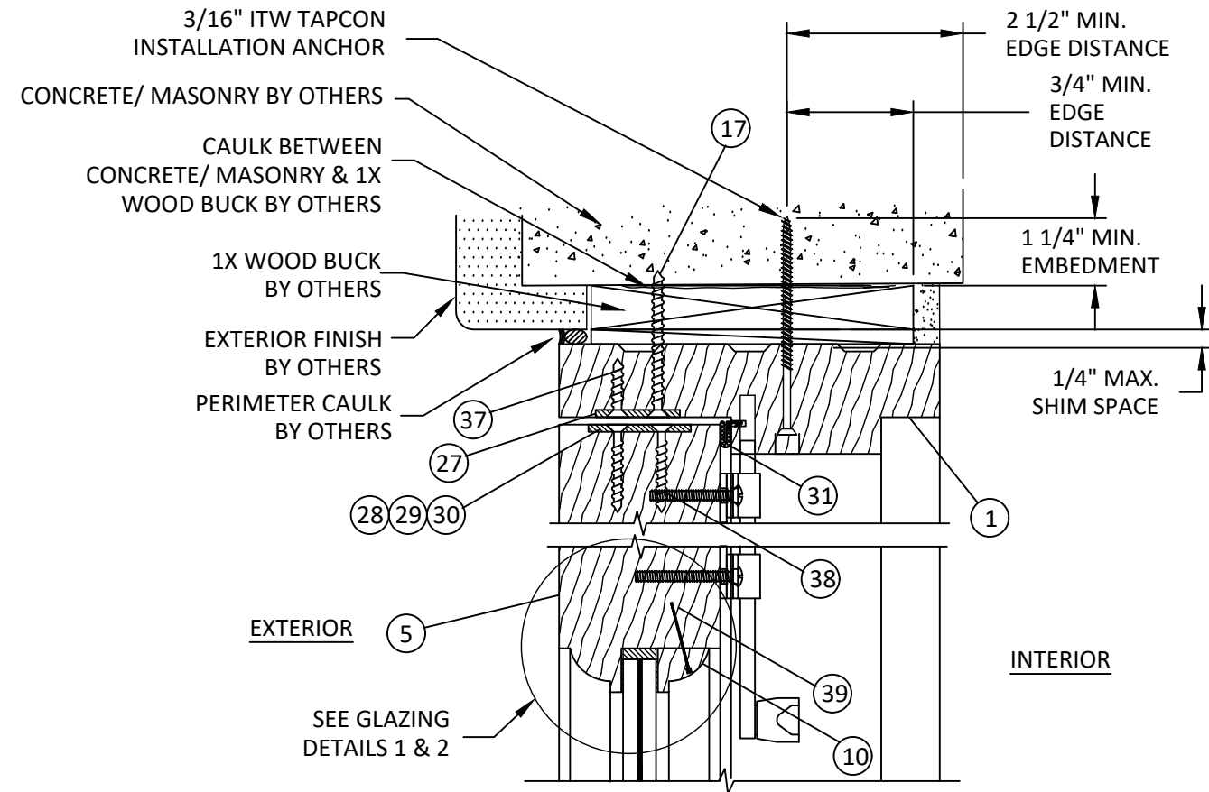
H 7 VERTICAL SECTION DOOR HEAD AT CONCRETE/MASONRY
