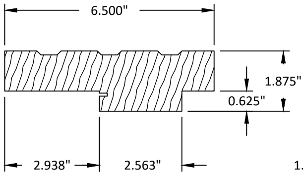
5 HINGE STILE AND TOP RAIL WOOD
