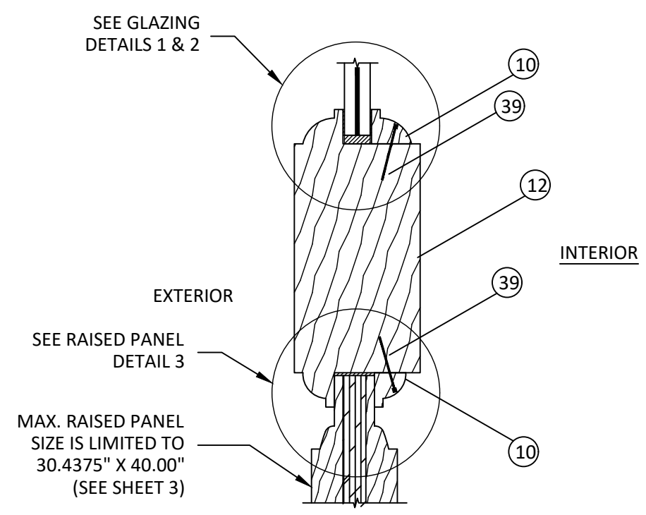
F 7 VERTICAL SECTION AT MID RAIL
