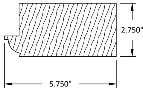
9 LOCKING STILE WOOD
