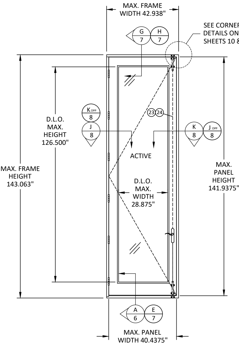
EXTERIOR ELEVATION (OUTSWING DOORS)
