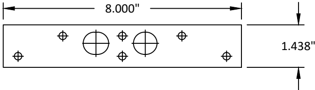
28 HINGE SIDE REINF. PLATE ALUMINUM
