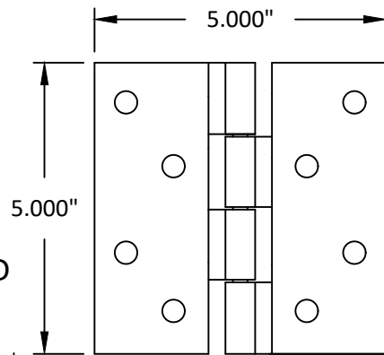
22 HINGE STEEL
