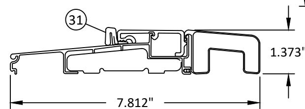
14 ENDURA BUMPER THRESHOLD EXTRUDED ALUMINUM
