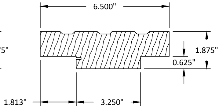
6 OFFSET HINGE STILE AND TOP RAIL WOOD
