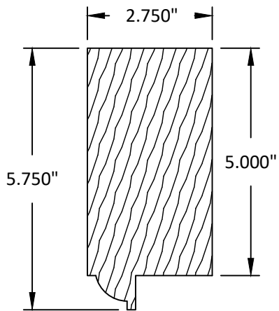
5 HINGE STILE AND TOP RAIL WOOD
