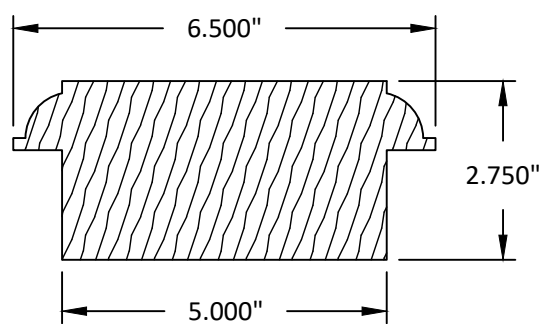
12 MID RAIL WOOD
