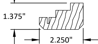
44 EXT. ASTRAGAL CAP WOOD
