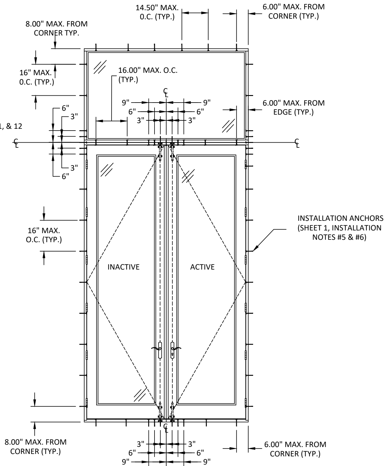
ANCHOR LAYOUT
