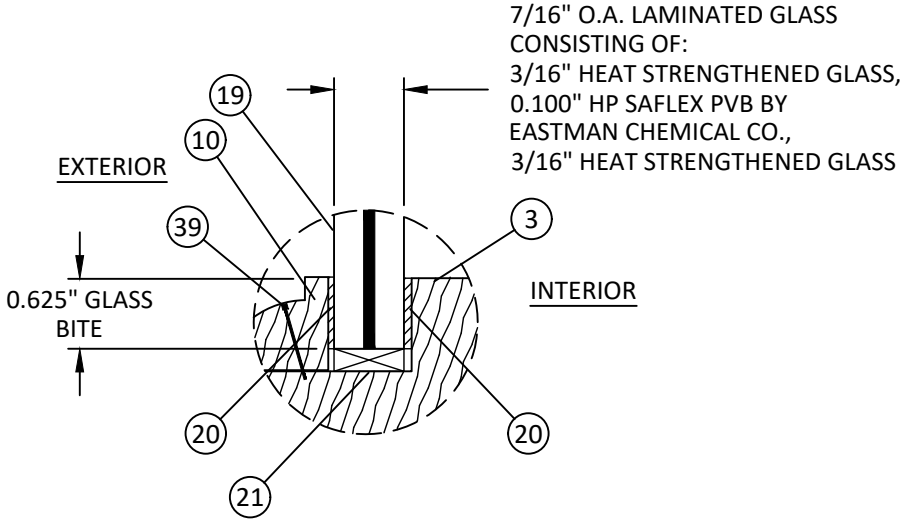
GLAZING DETAIL 2
