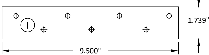
30 INACTIVE LOCK SIDE REINF. PLATE ALUMINUM
