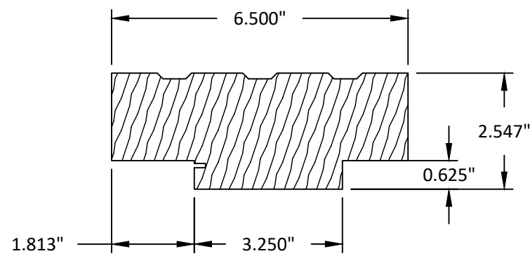
9 LOCKING STILE WOOD
