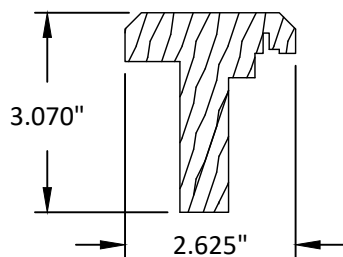
44 EXT. ASTRAGAL CAP WOOD
