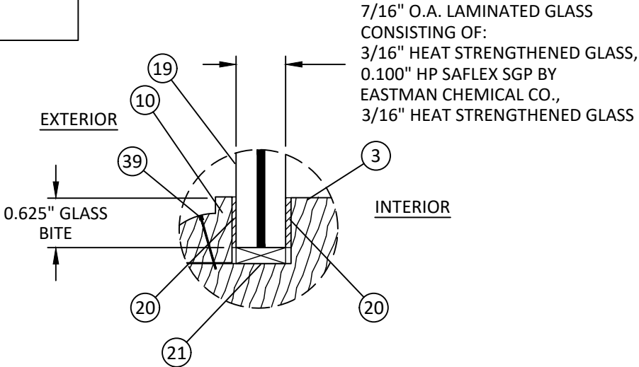
GLAZING DETAIL 4
